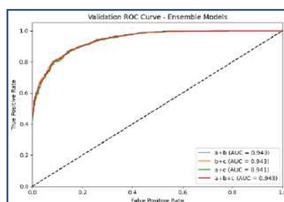
Figure 4.18: ROC-AUC Curve ( Validation)
