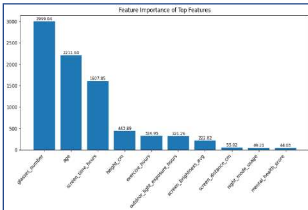
Fig 2: Feature Importance
