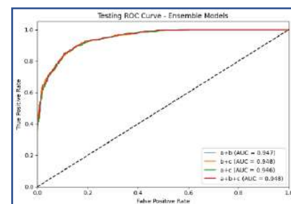
Figure 4.19: ROC-AUC Curve Testing
