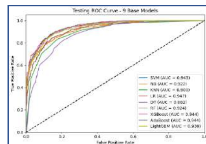
Figure 4.16: ROC-AUC Curve (Testing)
