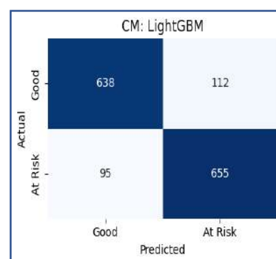
Fig 4.9 Confusion Matrix LightGBM
