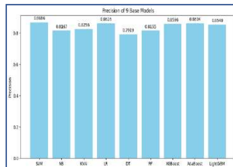
Fig 4.21: Precision of 9 Base Model
