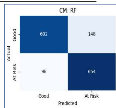
Fig 4.6 Confusion Matrix RF
