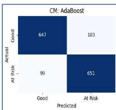
Fig 4.8 Confusion Matrix AdaBoost
